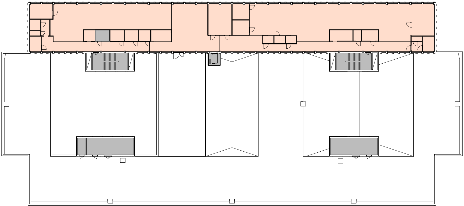
PLAN 12 BRA
