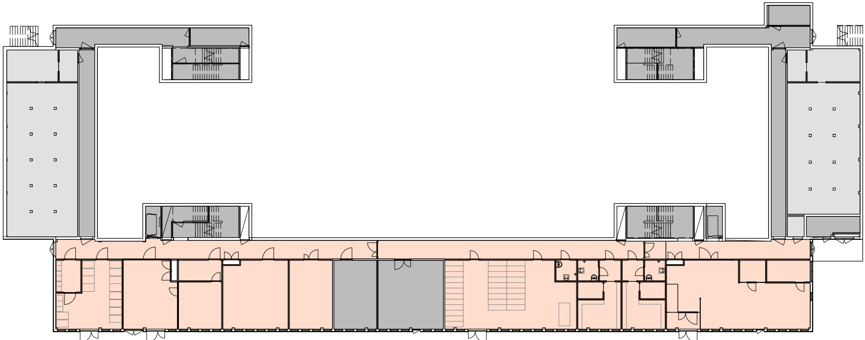
PLAN 09 BRA
